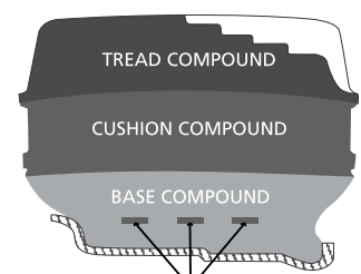
LIP TYPE TYRE
